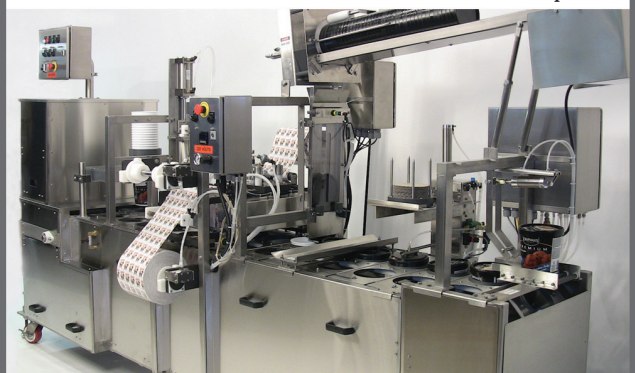
Automatic Dual Lane Filler with Membrane Seal for 5 to 64 ounce sizes
